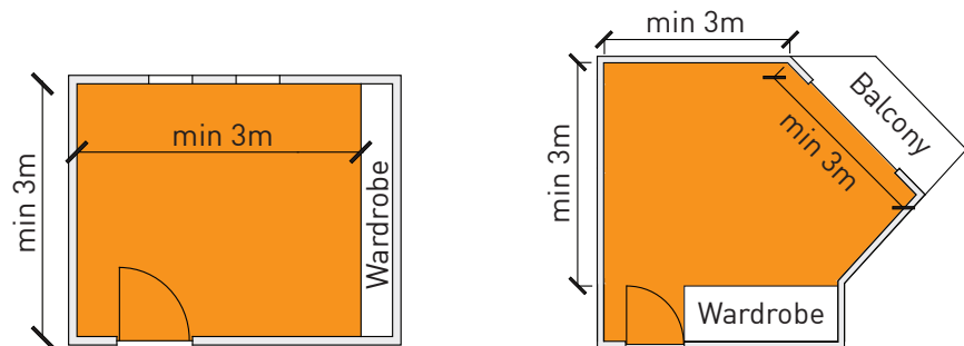
Figure 5C.4-1: Minimum plan dimension 3m x 3m for habitable rooms
