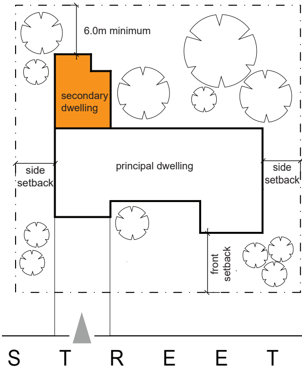
Figure 5A.3-1: Setback controls for attached secondary dwellings.
