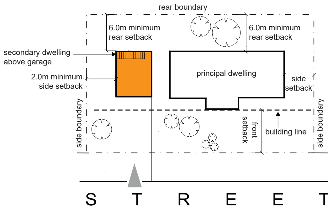
Figure 5A.3-3: Setback controls for secondary dwellings above a detached garage.
